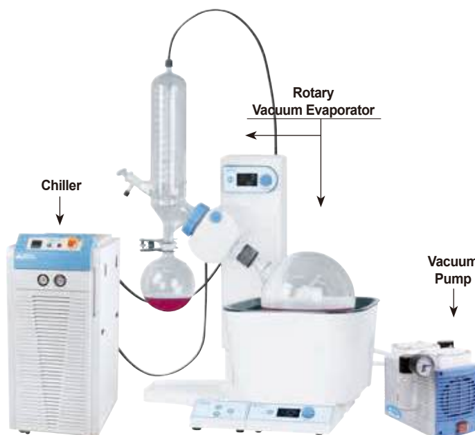
▶ Figure ; One of the Applications in the Large Volume Evaporator Line.
