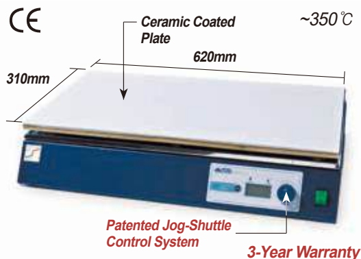
A. Large Digital Hotplate, with Built-in Digital PID Controller, Ceramic-Coated Plate-type “HPLP620”
