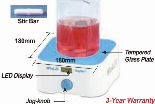
180×180mm Midi Magnetic Stirrer “MS-18D”
