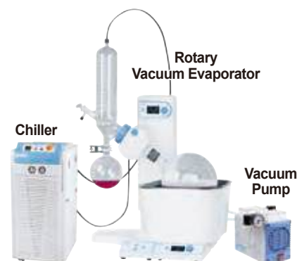
► Figure ; One of Rotary Vacuum Evaporator Systematization
