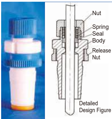
High Performance Shaft Guides
