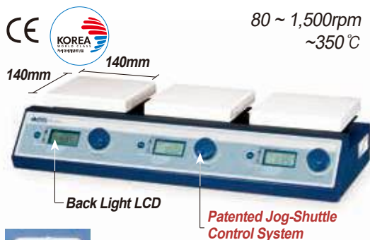
Stir Bar A. 3 Plate-type Multi-Hotplate Stirrer “SMHS-3”
