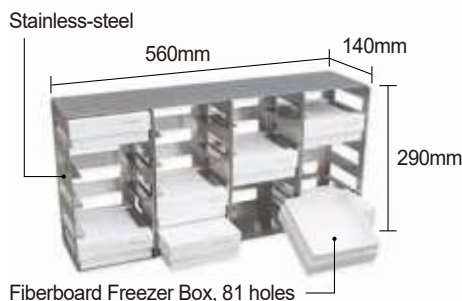
(2) Side Access-Type Rack, 20 Place "RFU4257SA"
