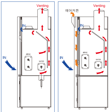
I. By-Pass Air Flow-type
