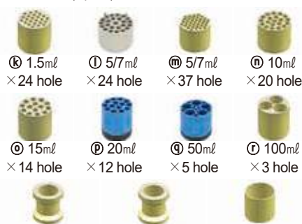
PP Adapters for (3) Rotor “R3-1000R”
