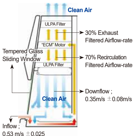
Safe Air Circulation System by EN12469 Standard
