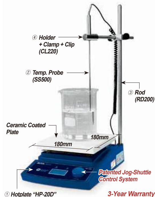
III-A. Digital Package Set “HP-20D” Set
