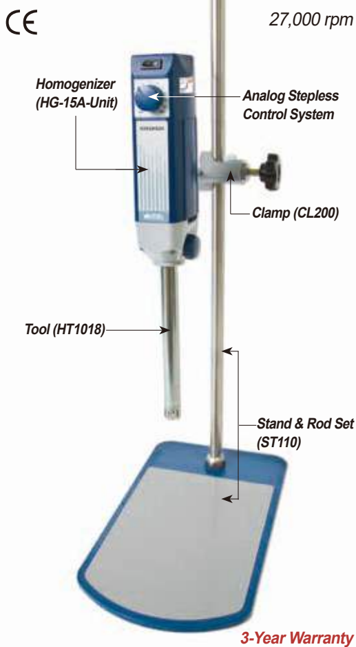
A. Homogenizer Package-set "HG-15A-SET-A"
