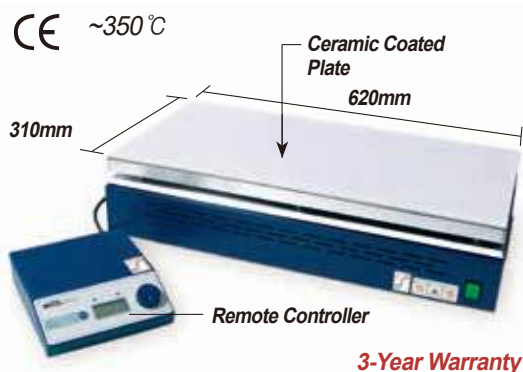
B. Large Digital Hotplate, Digital Remote Controller, Ceramic-Coated Plate-type “HPLP620R”
