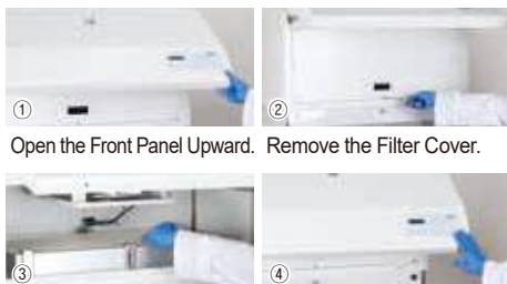
Remove the Filters in order, then Install the New Filters in Reverse Order. Reassemble the Filter Cover and Close the Front Panel.
