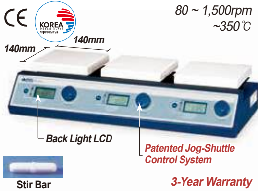
A. 3 Plate-type Multi-Hotplate Stirrer “SMHS-3”
