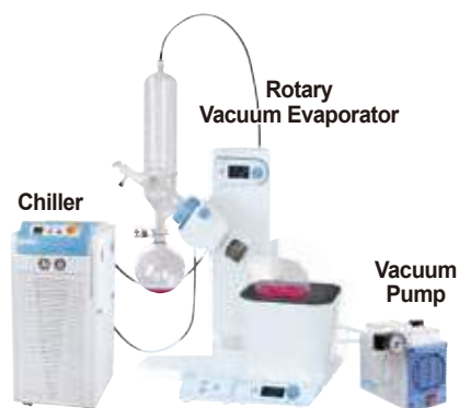
▶ Figure ; One of Rotary Vacuum Evaporator Systematization
