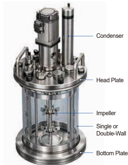
BIOPRIME™ Complete Vessel
