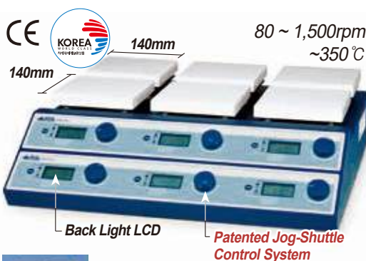
Stir Bar B. 6(3×2) Plate-type Multi-Hotplate Stirrer “SMHS-6”
