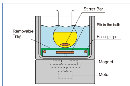
Drawing of “MBWCL-3”
