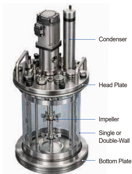
BIOPRIME™ Complete Vessel
