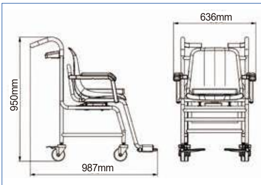
Dimension Drawing
