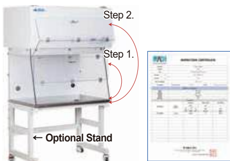
Fig. 11° Slanted 2-Step Folding Window & Optional Stand
