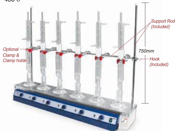
6 places Heating Mantle (WHM12293)
