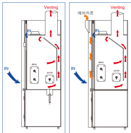
I. By-Pass Air Flow-type
